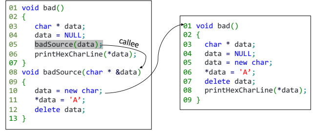
(a) Example for SARD dataset with the root cause of vulnerability in callee function
